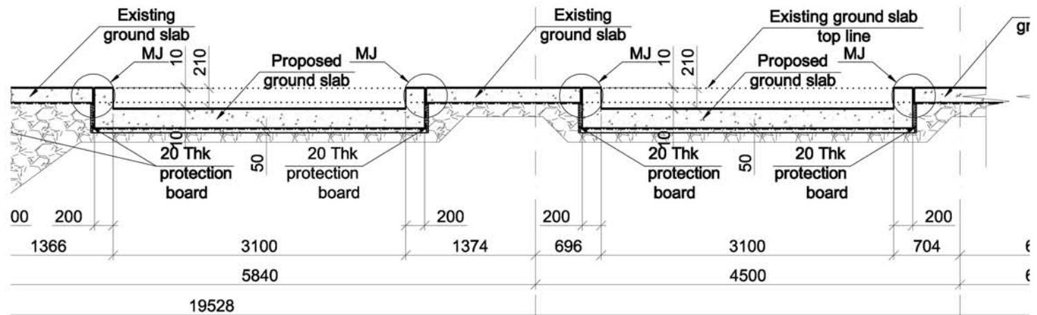
PROPOSED GROUND SLAB SECTION 3-3 Scale 1:50
